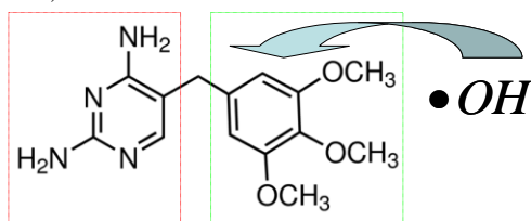
Figure 6. Preferential attack of \cdot\text{OH} to TMP
