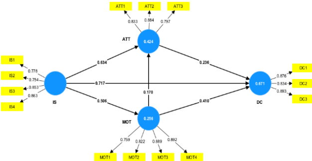
Figure 1. Results of PLS-SEM Analysis
